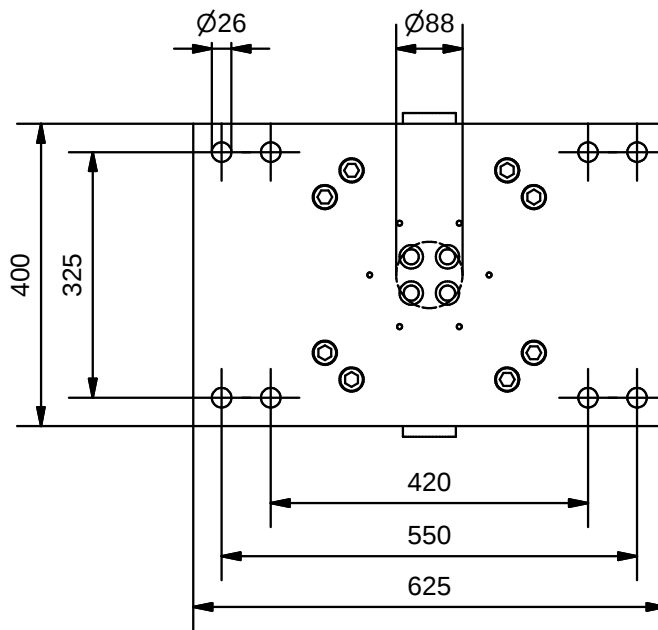
Bottom view (1:10)
